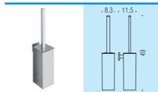
B3707 Porta scopino da parete Wall mounted brush holder
