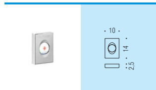
B9982 Porta sacchetti igienici in ABS cromato ABS dispenser for sanitary bags
